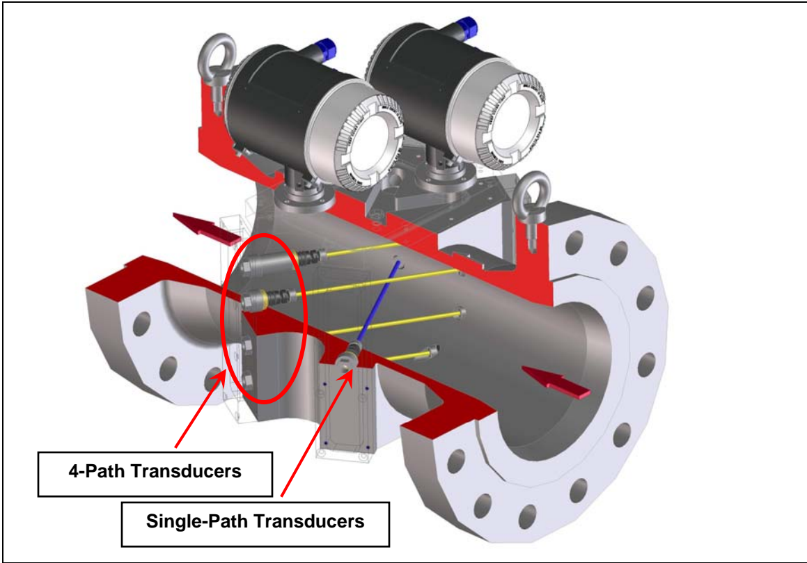
Figure 1: CBM 2Plex 4+1 Meter Design
