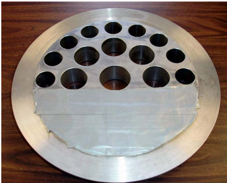
Figure 6: 12-inch CPA with 40% Blockage
