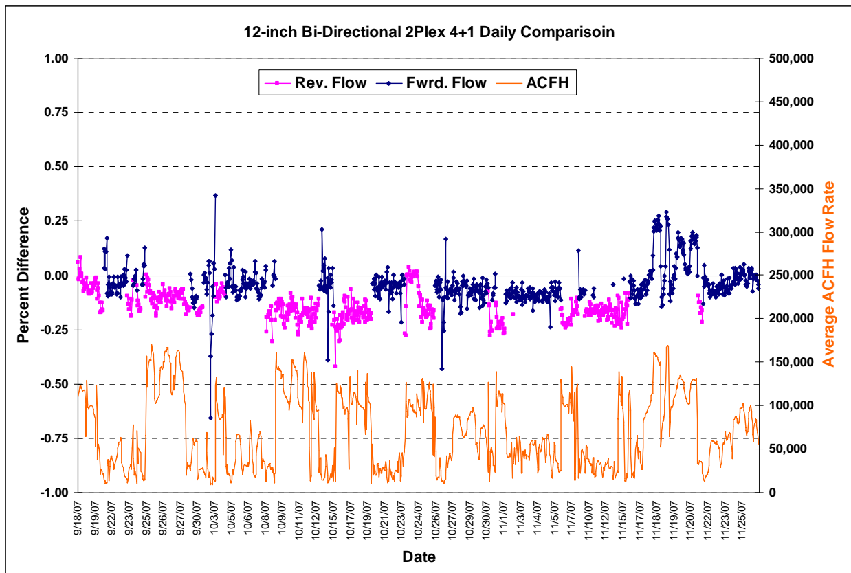
Figure 24: 4-Path vs. 1-Path Daily Comparison
