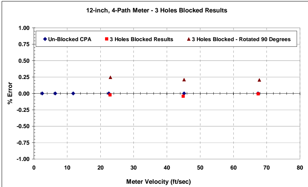
Figure 10: 12-inch, 4-Path Meter Results with 3 Holes Blocked
