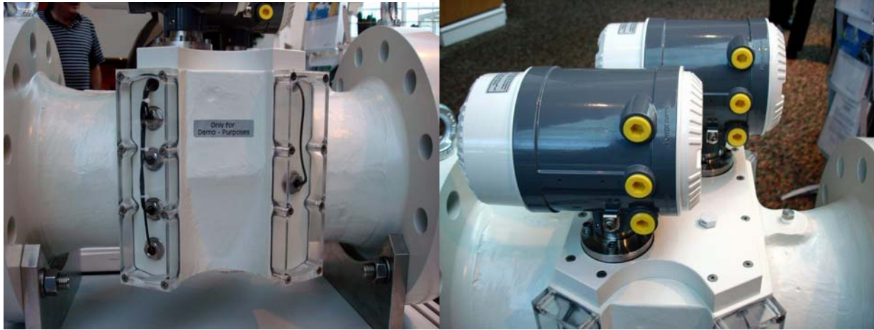
Figure 3: CBM 2Plex 4+1 Transducers
