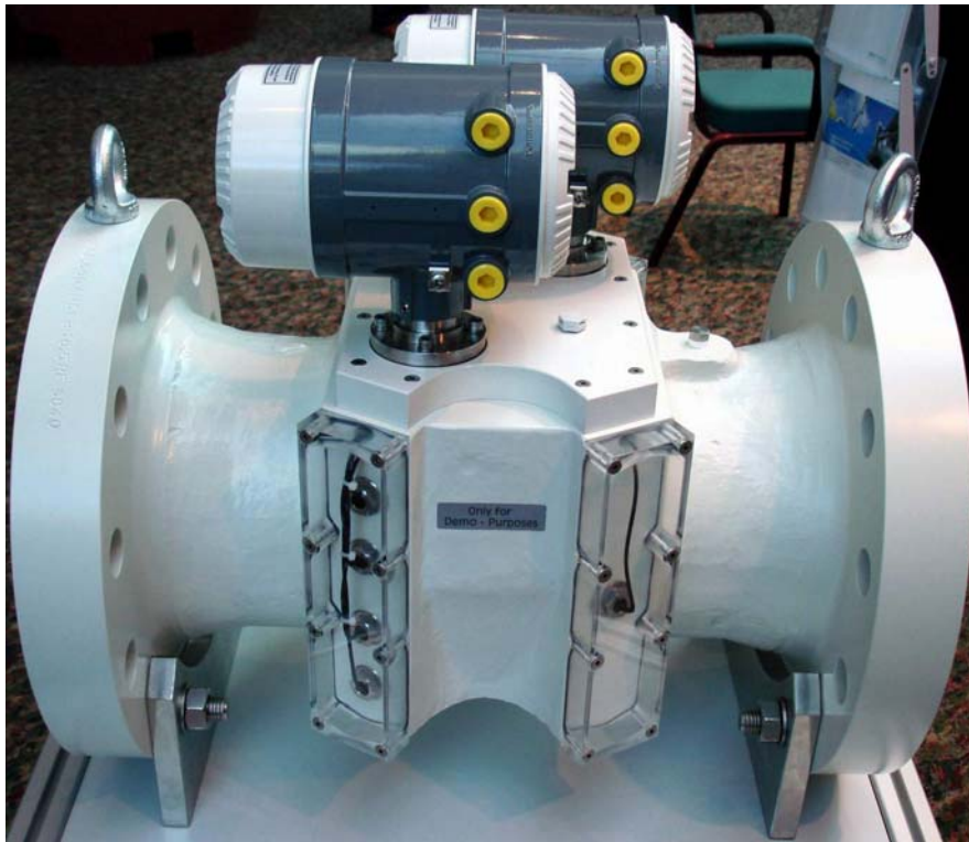
Figure 2: 8-inch CBM 2Plex 4+1-Path Meter
