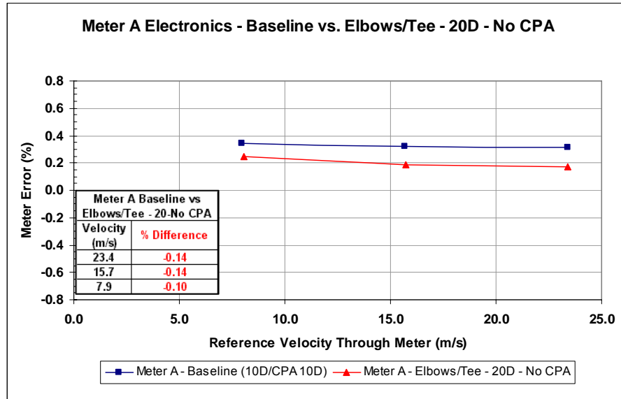
Figure 23: Meter A Results – 20D No CPA
