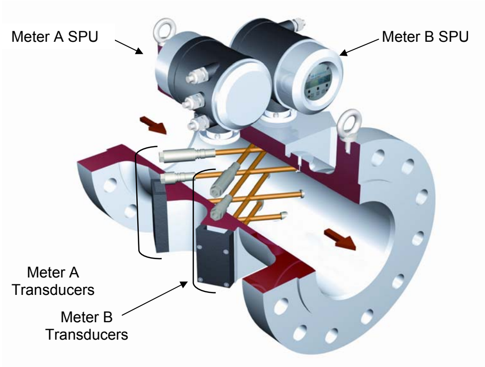
Figure 1: 8-Path Meter Used for Testing
