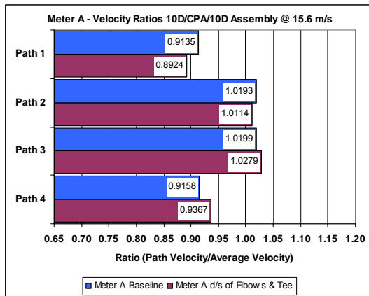
Figure 18: Meter A Velocity Ratios – Baseline vs. Disturbed Flow
