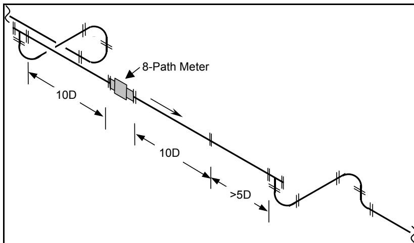
Figure 14: 10D – No Flow Conditioner Test Run Assembly
