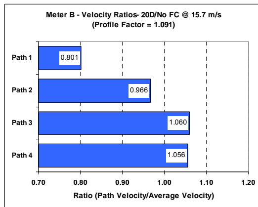
Figure 22: Meter B Profile for 20D – No CPA
