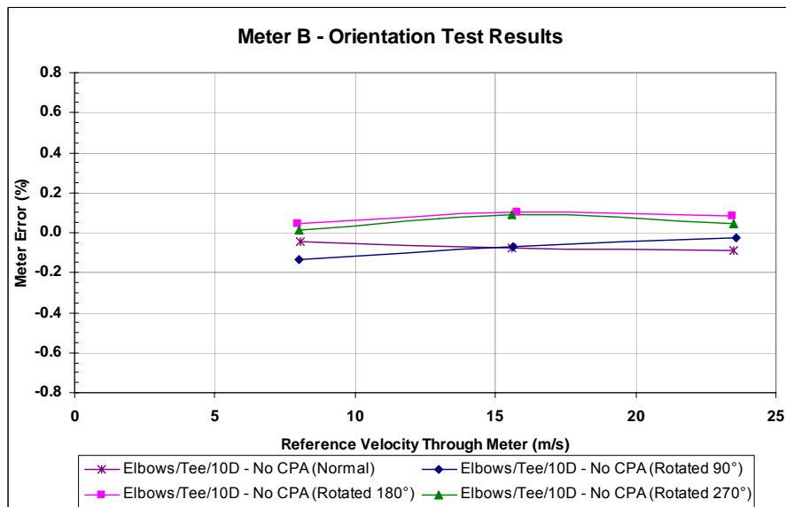
Figure 35: Meter B Error As a Function of Radial Orientation
