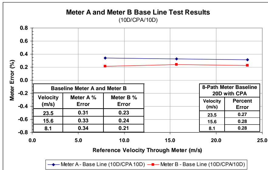
Figure 5: Baseline Test Results
