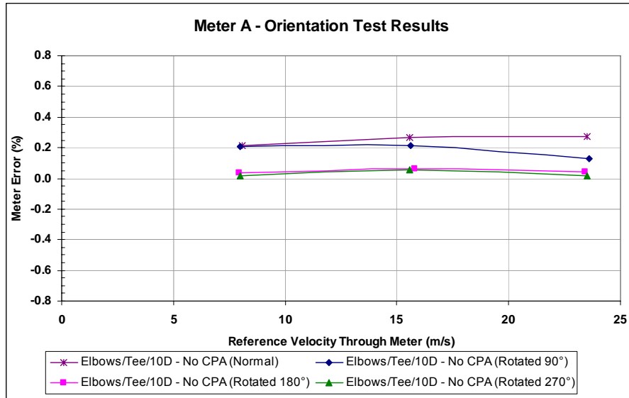
Figure 34: Meter A Error As a Function of Radial Orientation
