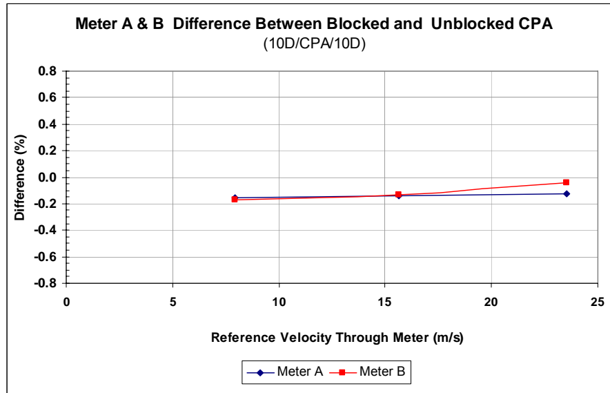
Figure 9: Meter Error – Blocked Conditioner vs. Baseline
