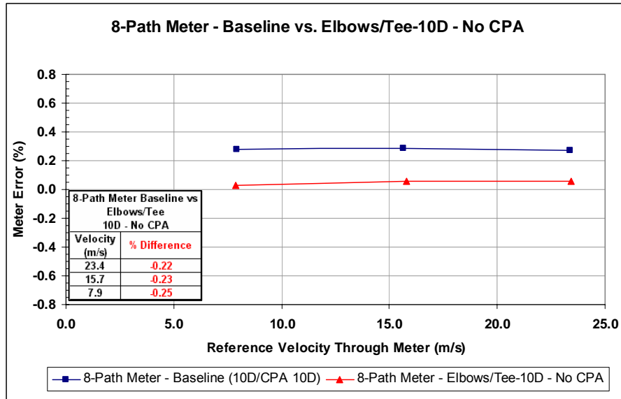
Figure 29: 8-Path Meter at 10D No Flow Conditioner
