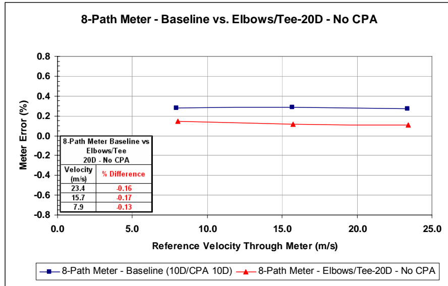
Figure 25: 8-path Meter Results – 20D No CPA
