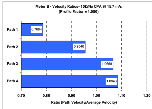
Figure 31: Meter B Profile at 10D – No CPA
