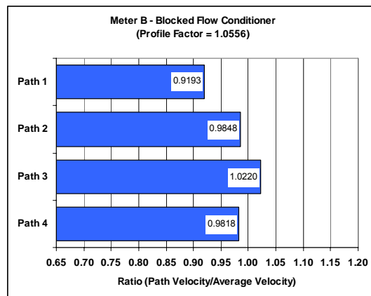
Figure 8: Meter B – Velocity Ratios with Blocked Flow Conditioner
