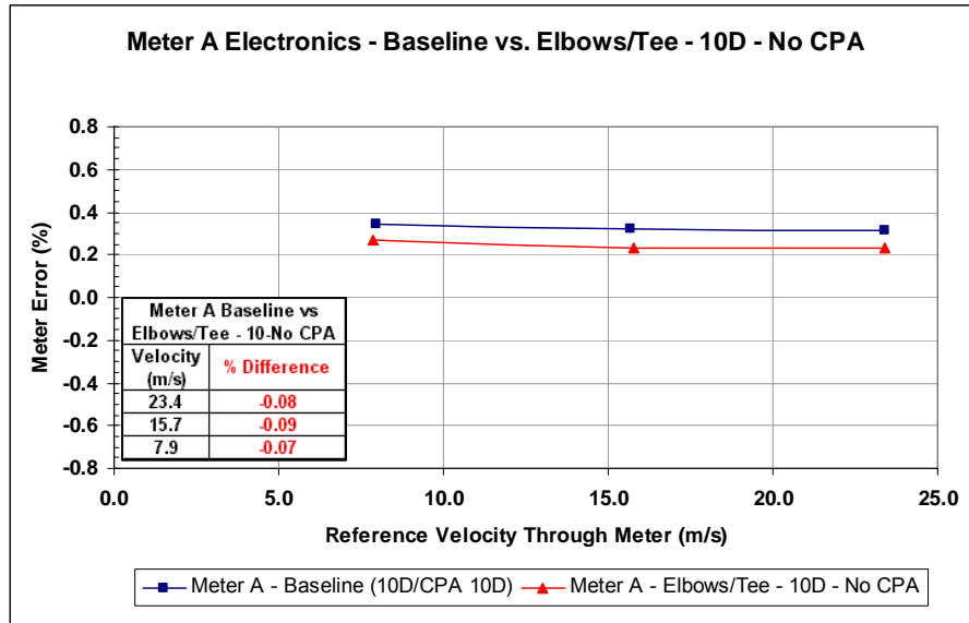
Figure 27: Meter A at 10D No Flow Conditioner
