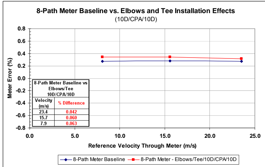
Figure 20: 8-Path Meter Performance with Tee and Elbows, 10D/CPA/10D
