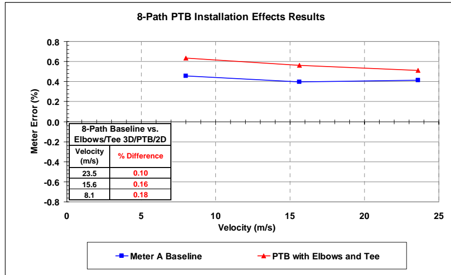
Figure 41: PTB Flow Conditioner Downstream of Elbows and Tee
