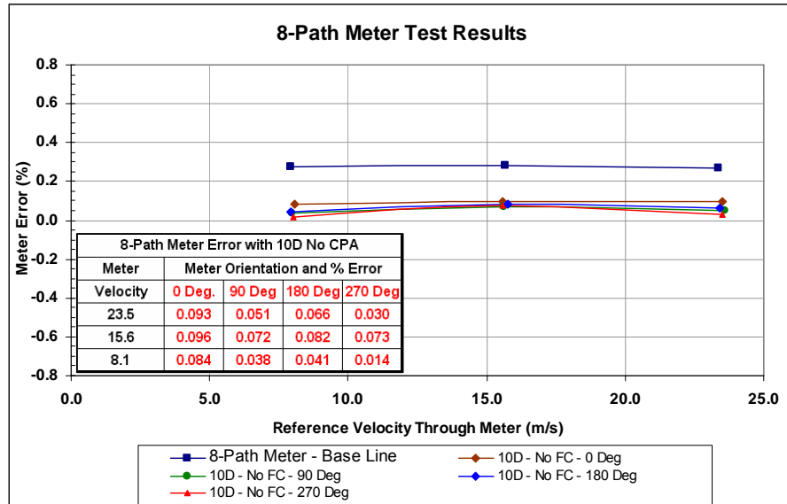
Figure 36: 8-Path Meter Error As a Function of Radial Orientation
