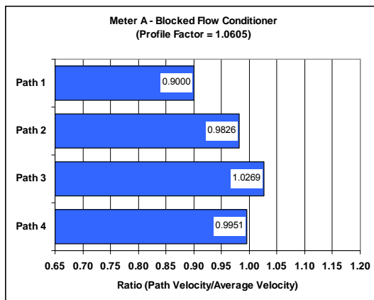
Figure 7: Meter A – Velocity Ratios with Blocked Flow Conditioner
