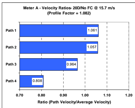
Figure 21: Meter A Profile for 20D – No CPA
