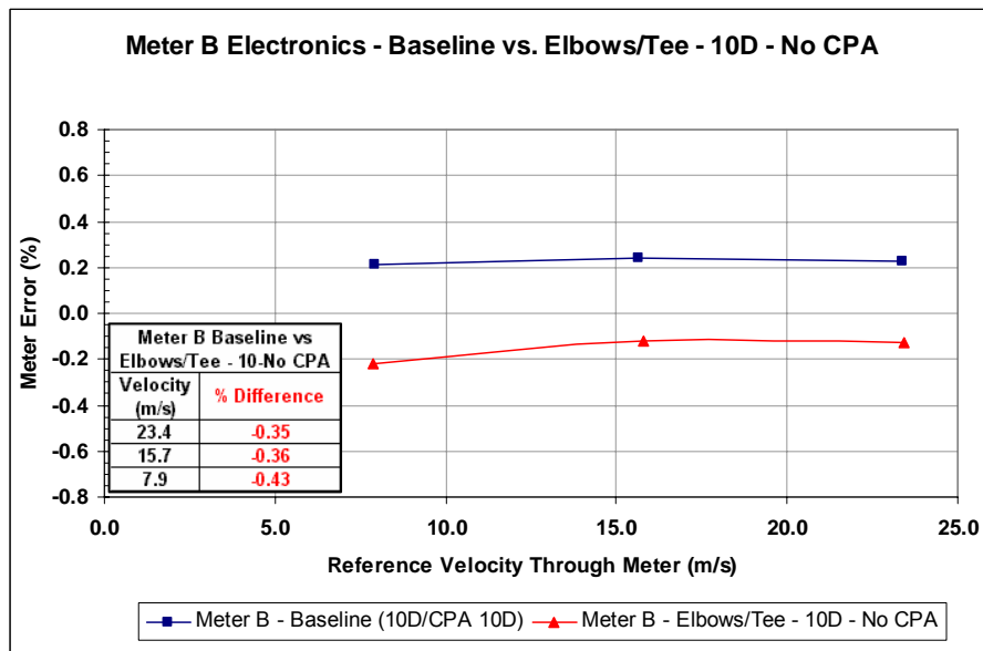
Figure 28: Meter B at 10D No Flow Conditioner
