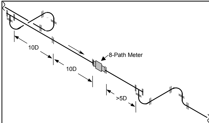
Figure 13: 20D – No Flow Conditioner Test Run Assembly
