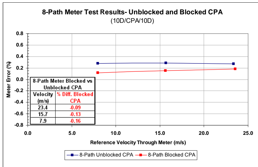
Figure 10: Meter Error – 8-Path Results
