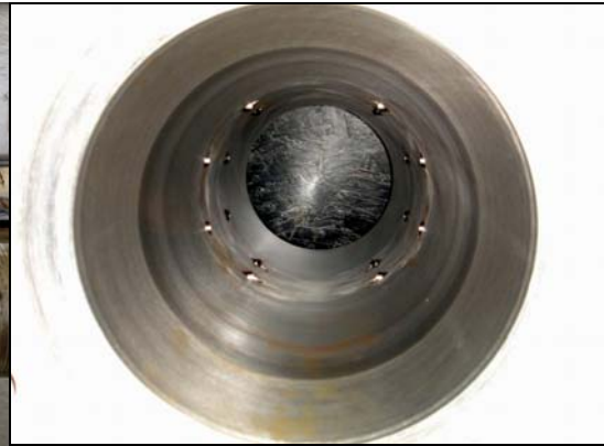
Figure 3: 8-Path Meter – Transducers
