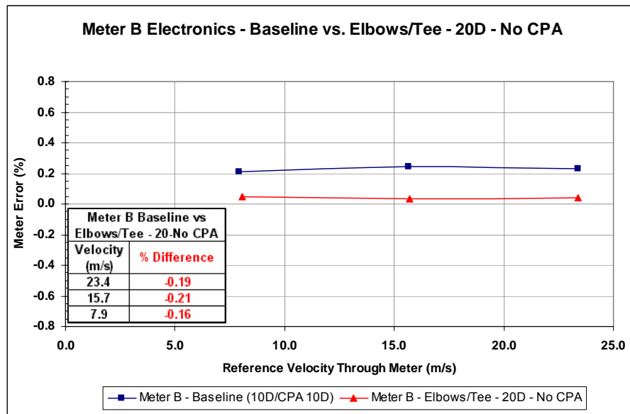
Figure 24: Meter B Results – 20D No CPA
