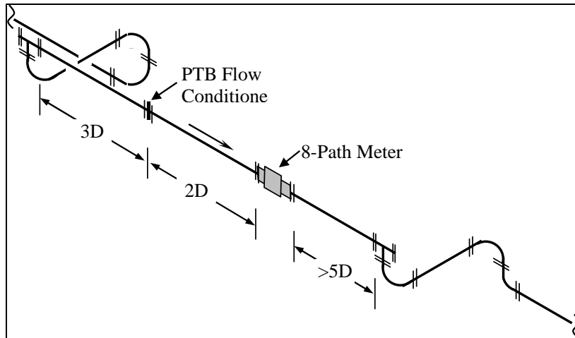
Figure 39: 3D/PTB/2D Flow Conditioner Piping
