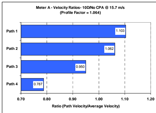
Figure 30: Meter A Profile at 10D – No CPA
