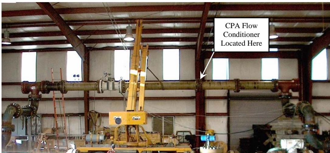
Figure 15: Picture of 10D/CPA/10D Installation
