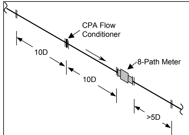
Figure 4: Meter Run Assembly for Baseline Testing
