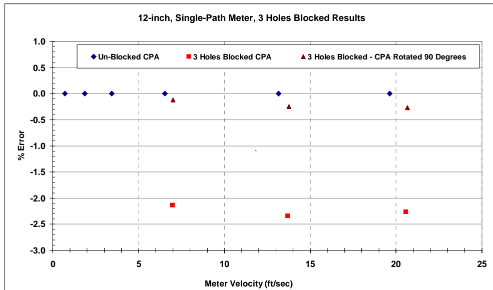
Figure 11: 12-inch, Single-Path Meter Results with 3 Holes Blocked
