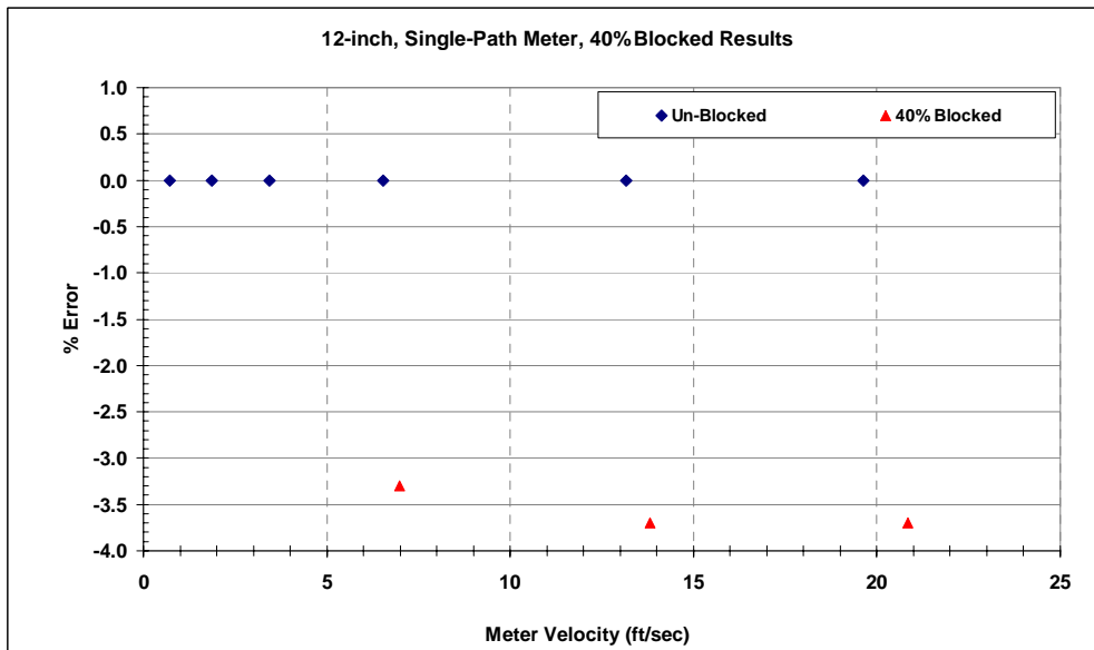
Figure 8: 12-inch, single-Path Meter Results with 40% Blockage
