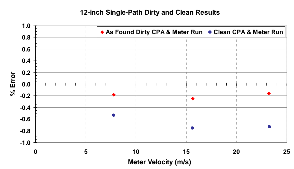
Figure 22: 12-inch, 4-path As-Found Dirty and As-Found Clean
