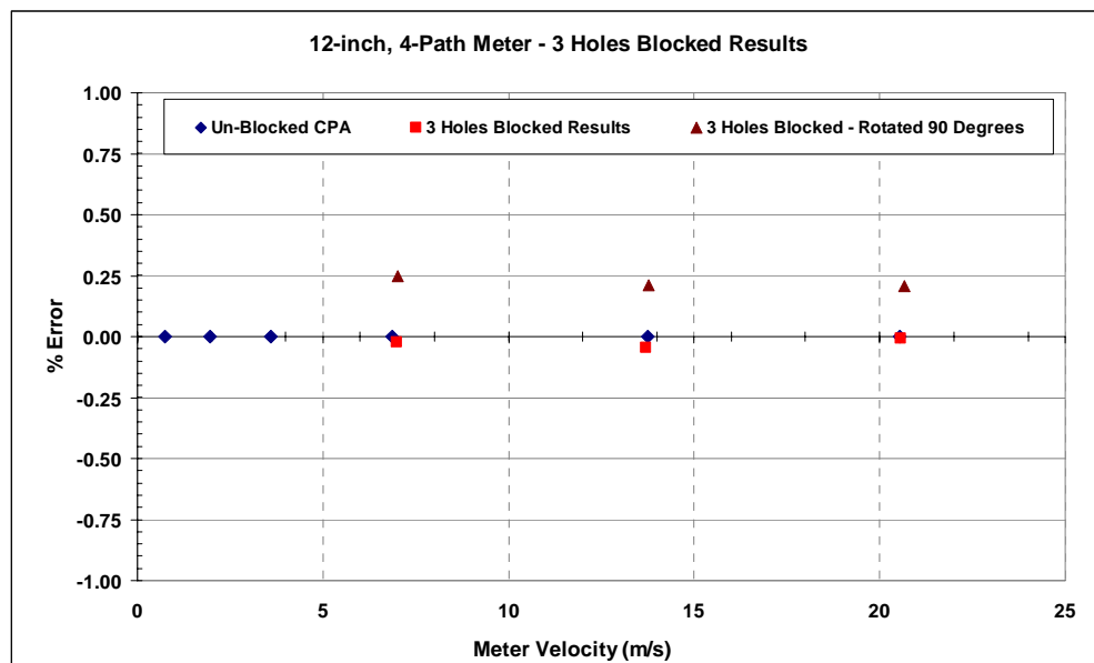
Figure 10: 12-inch, 4-Path Meter Results with 3 Holes Blocked
