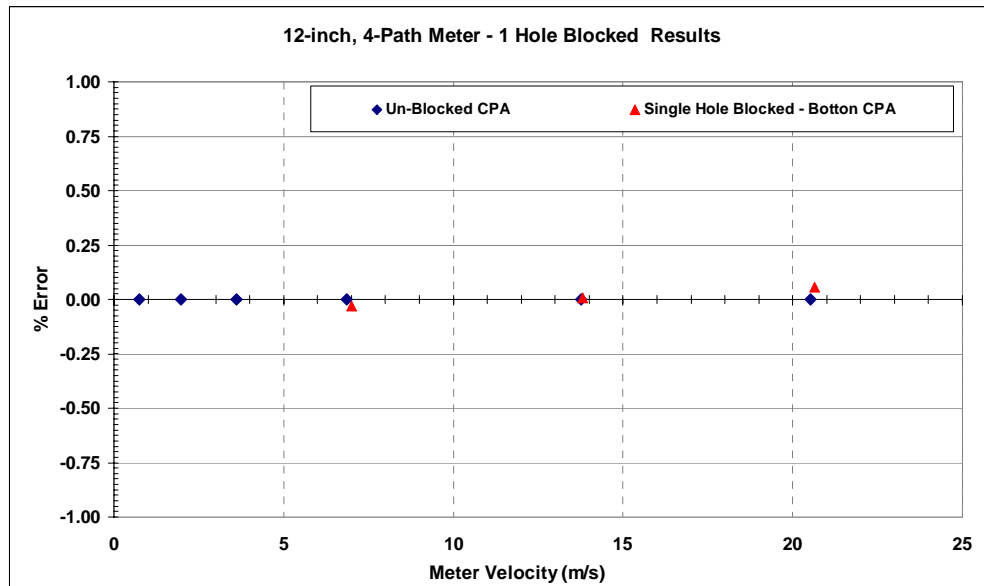
Figure 13: 12-inch, 4-Path Meter Results with 1 Hole Blocked
