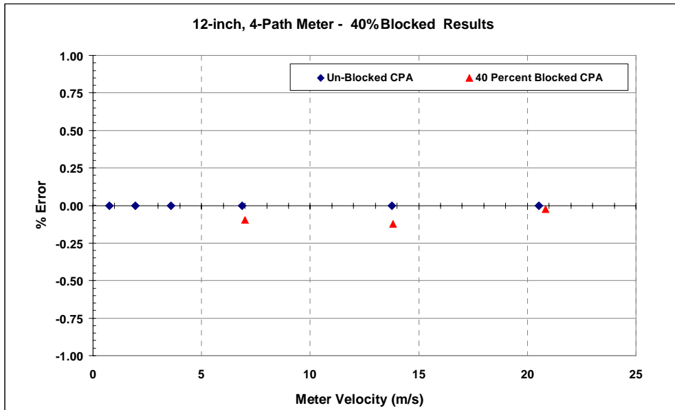
Figure 7: 12-inch, 4-Path Meter Results with 40% Blockage
