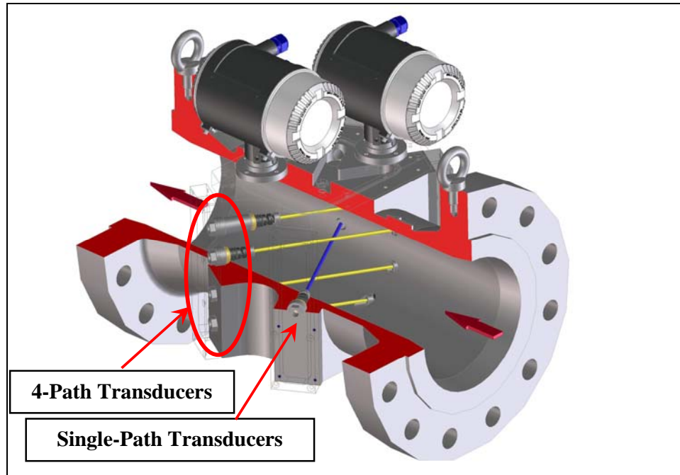
Figure 1: CBM 4+1 Meter Design
