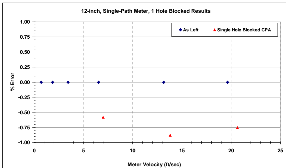
Figure 14: 12-inch, Single-Path Meter Results with 1 Hole Blocked
