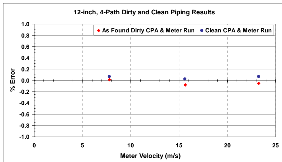
Figure 20: 12-inch, 4-path As-Found Dirty and As-Found Clean
