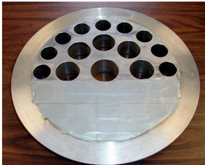
Figure 6: 12-inch CPA with 40% Blockage
